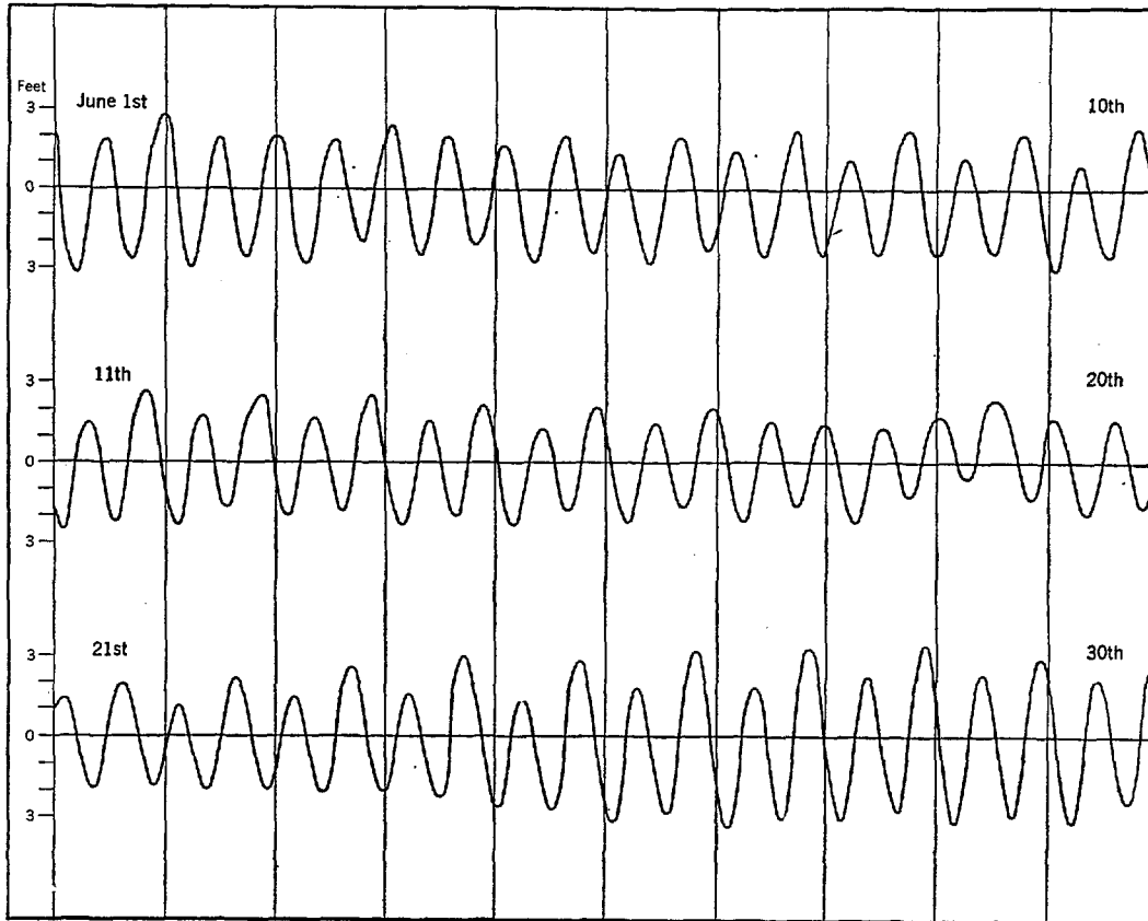
FIG. 4.—Tide curve, New York, June 1934.
