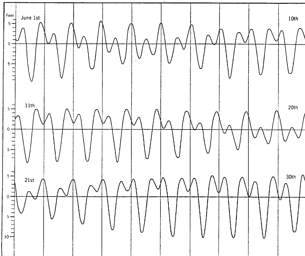
FIG. 7.—Tide curve, Seattle, June 1934.
