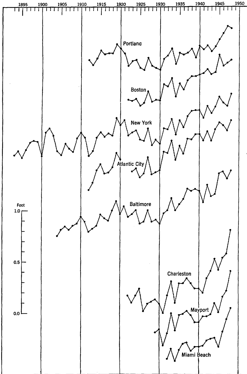
FIG. 20.—Yearly sea level, Atlantic coast.
