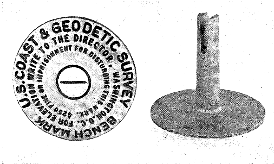
FIG. 10.—Standard tidal bench mark, United States Coast and Geodetic Survey†
