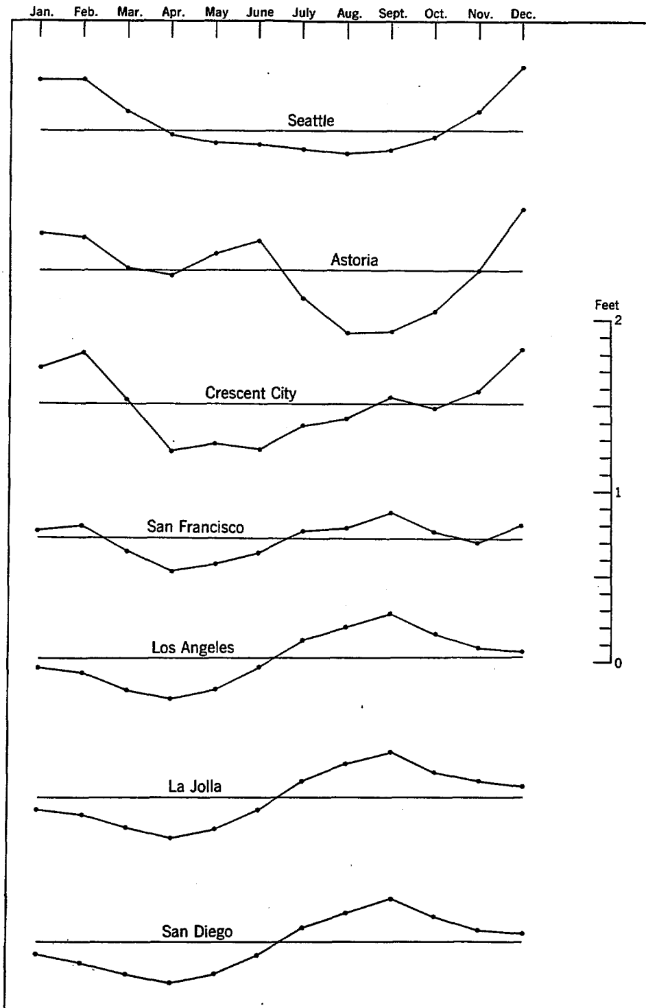
FIG. 23.—Annual variation in sea level, Pacific coast.
