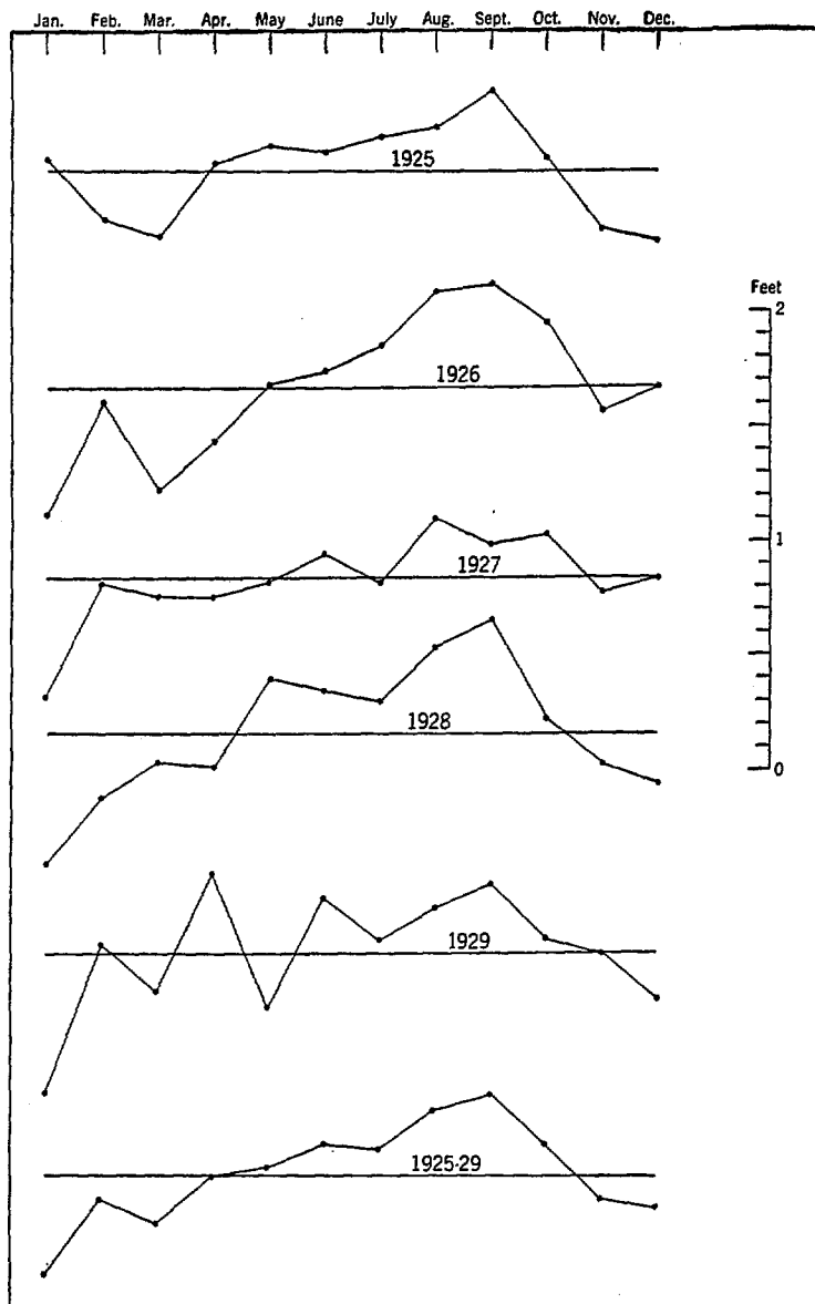
FIG. 25.— Annual variation in sea level, Atlantic City, 1925-29.
