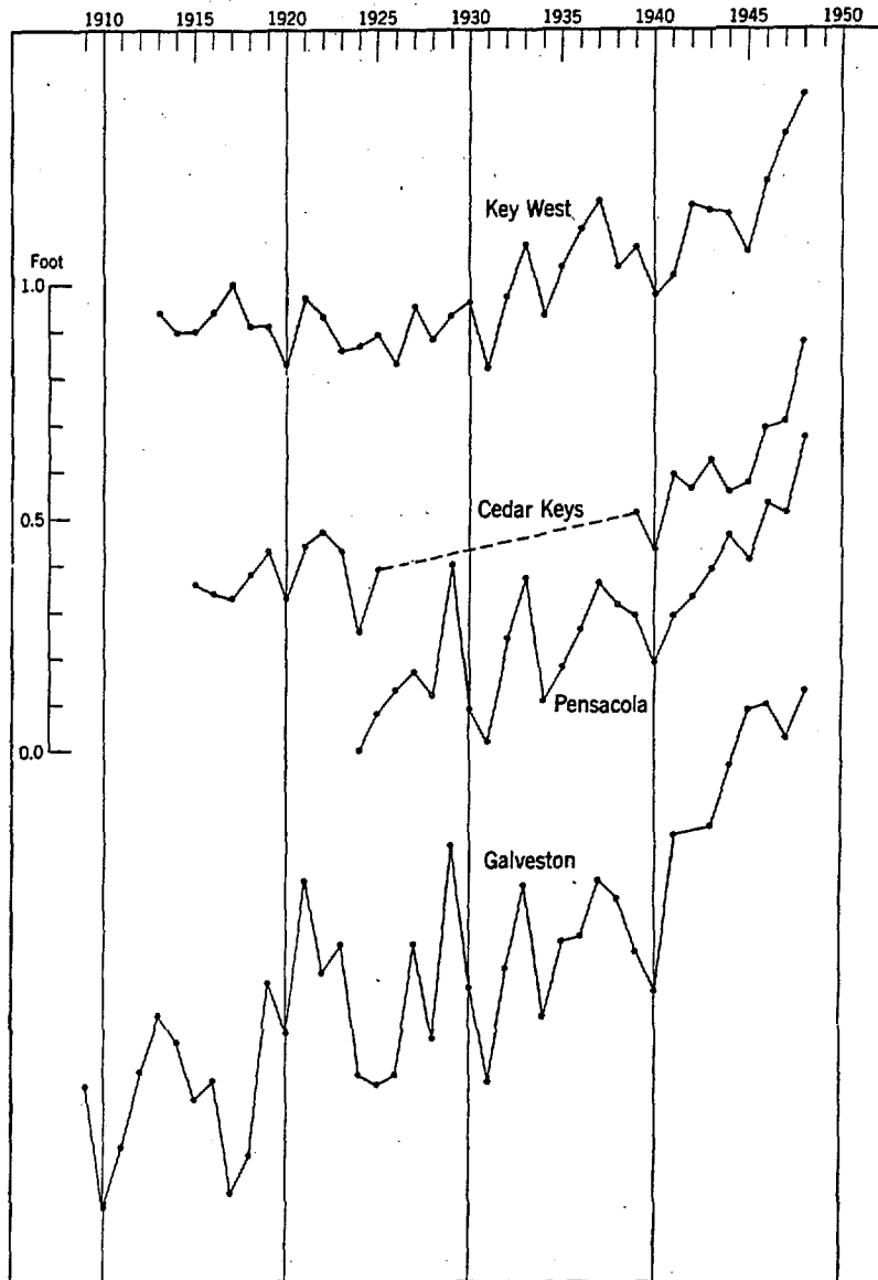
FIG. 31.—Yearly sea level, Gulf coast.
