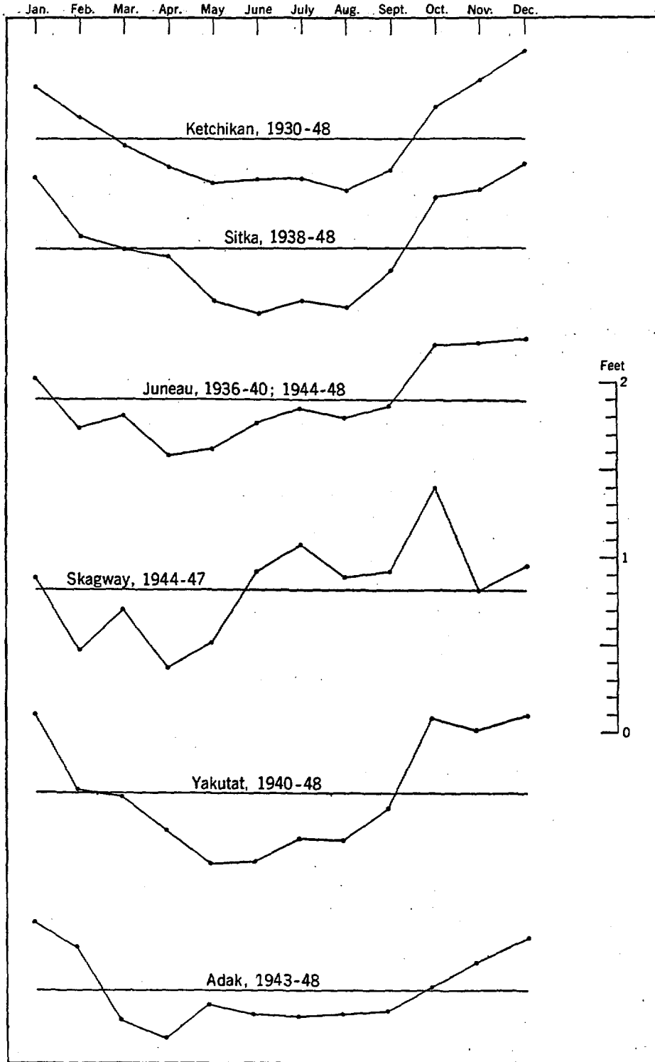
FIG. 29.—Annual variation in sea level, Alaska.
