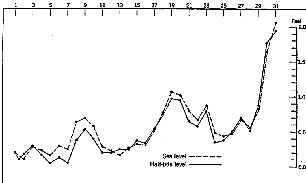
[Fig. 34.—Daily sea level and half-tide level, Boston, October 1947.]
