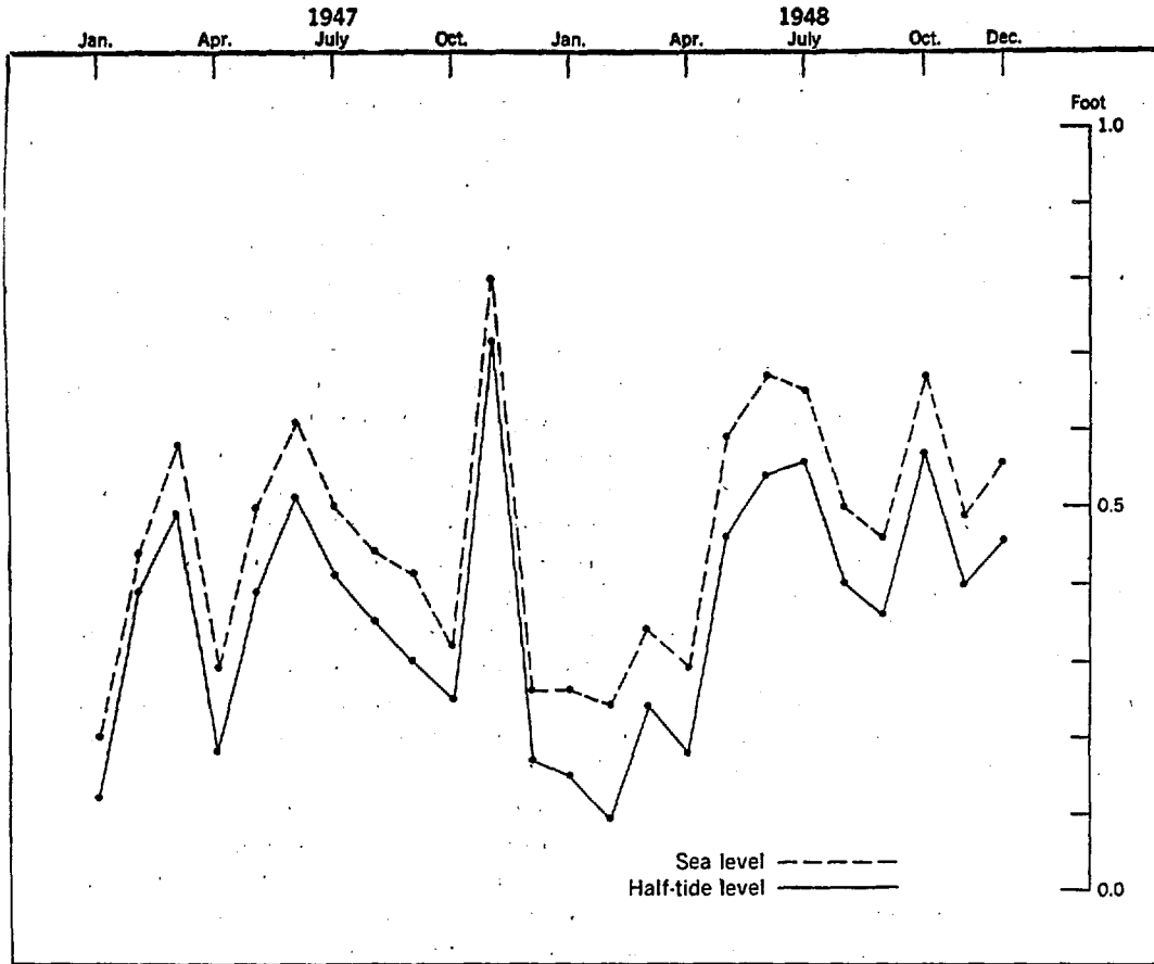
FIG. 35.—Monthly sea level and half-tide level, Boston, 1947-48.
