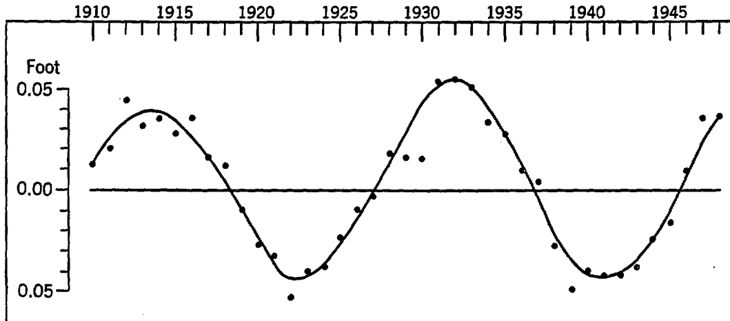
FIG. 37.—Relation of half-tide level to sea level, Seattle.
