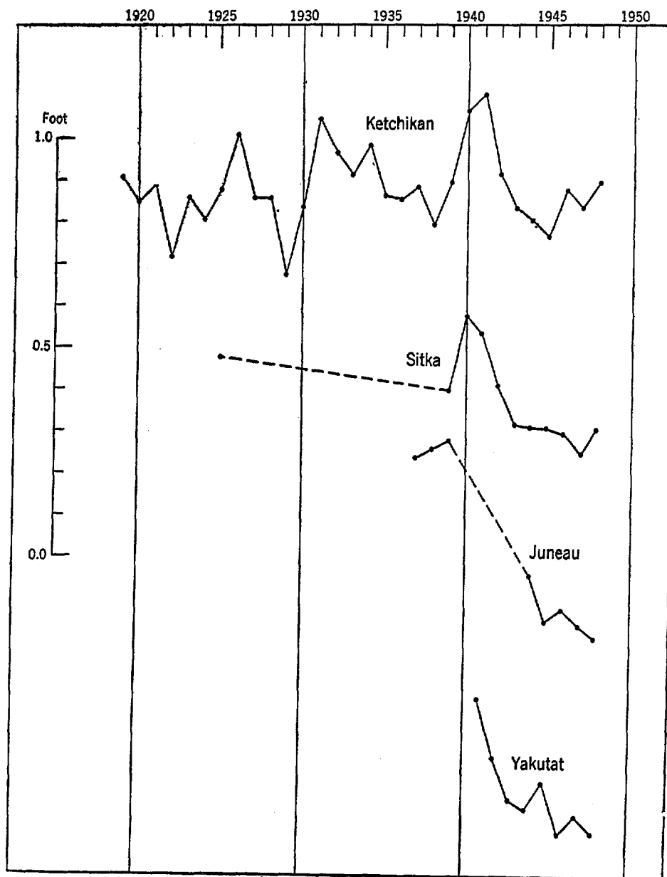
FIG. 33.—Yearly sea level, Alaska.
