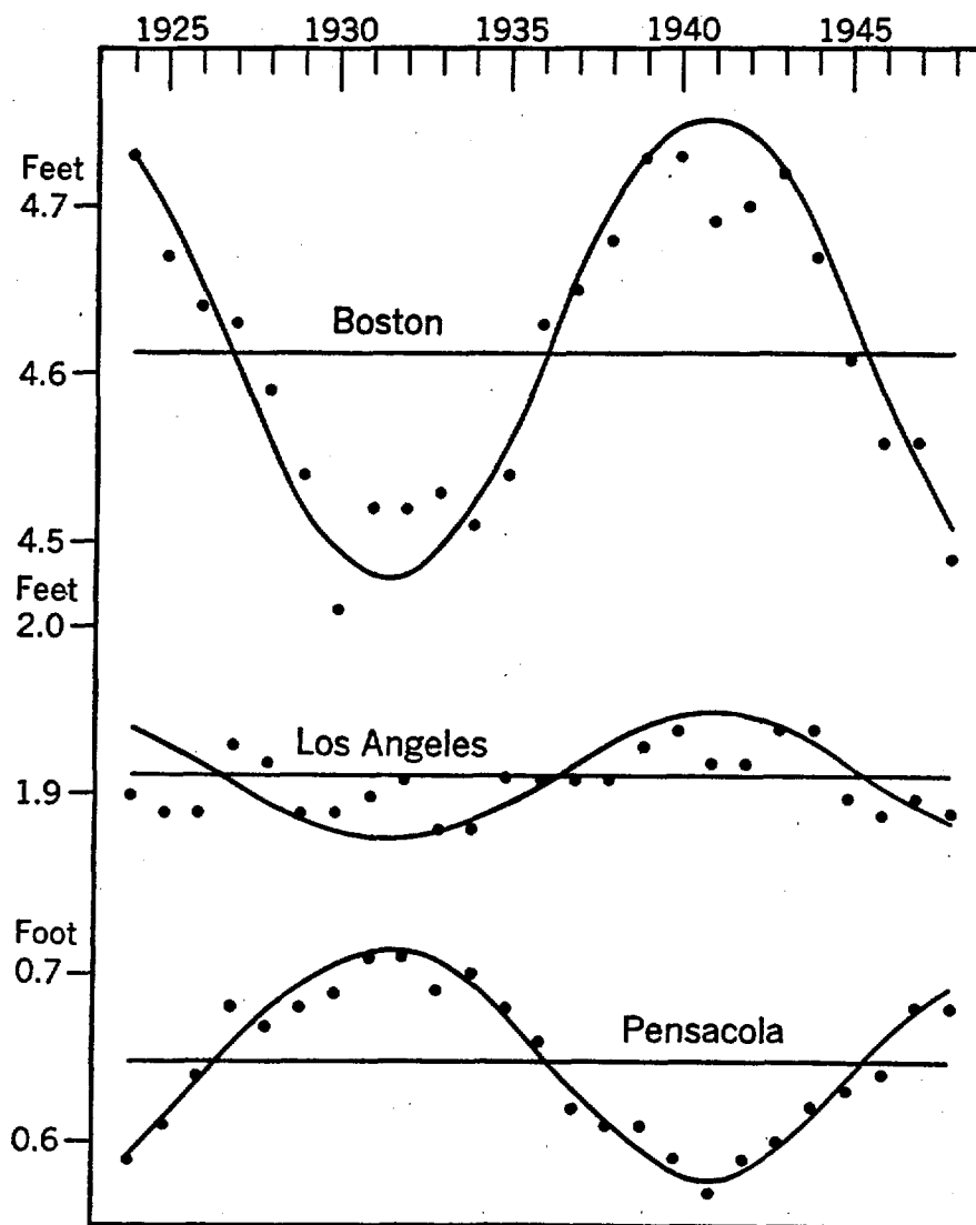
FIG. 43.—Variation of yearly high water in relation to yearly sea level.
