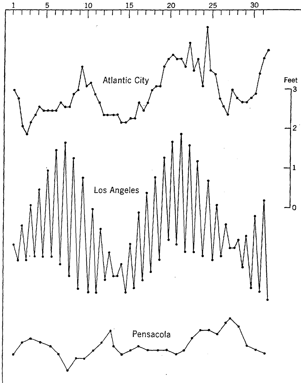
FIG. 44.—Low waters, Atlantic City, Los Angeles, and Pensacola, October 1947.
