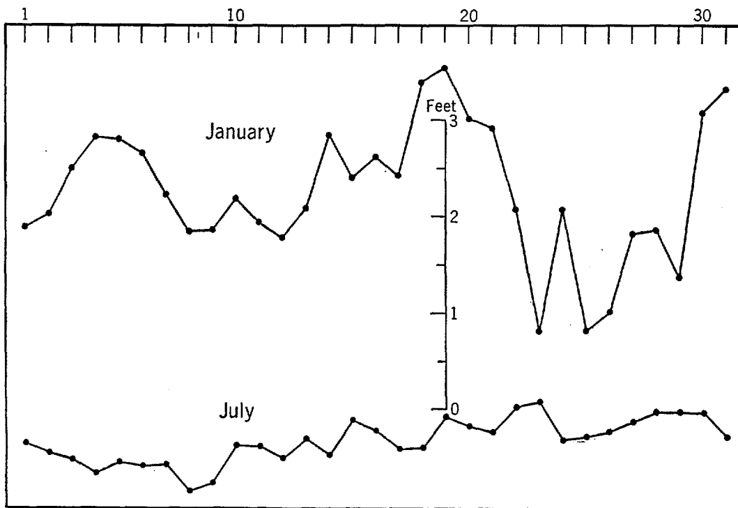
FIG. 22.—Daily sea level, Atlantic City, January and July 1939.
