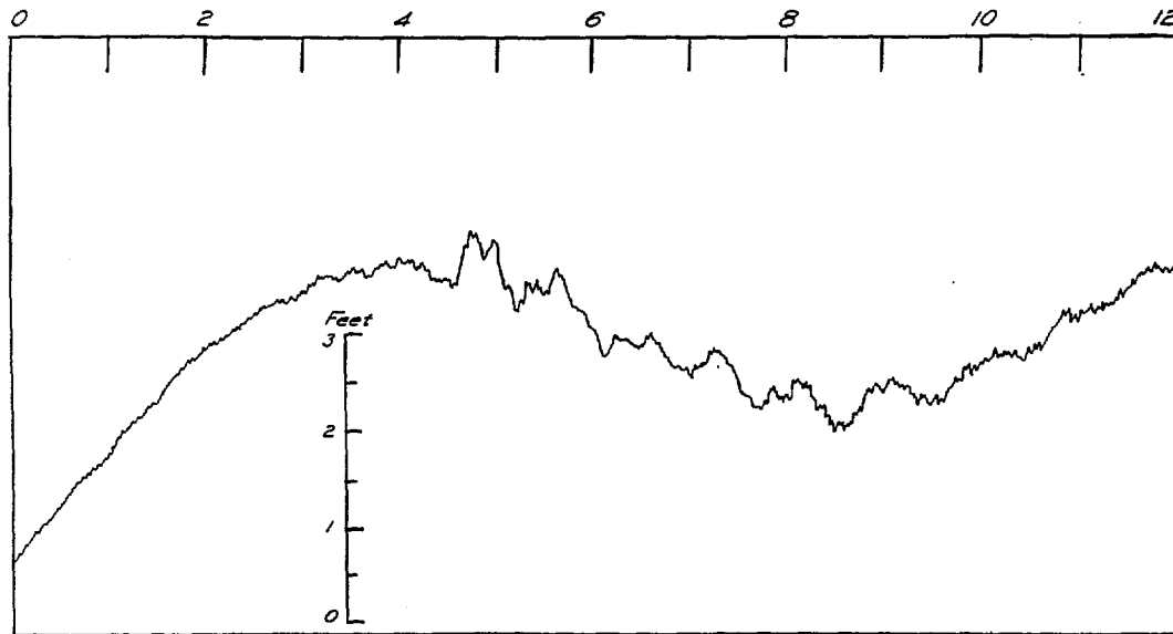
FIG. 18.—Tide curve, San Francisco, Calif., showing seiches due to changes in barometric pressure.
